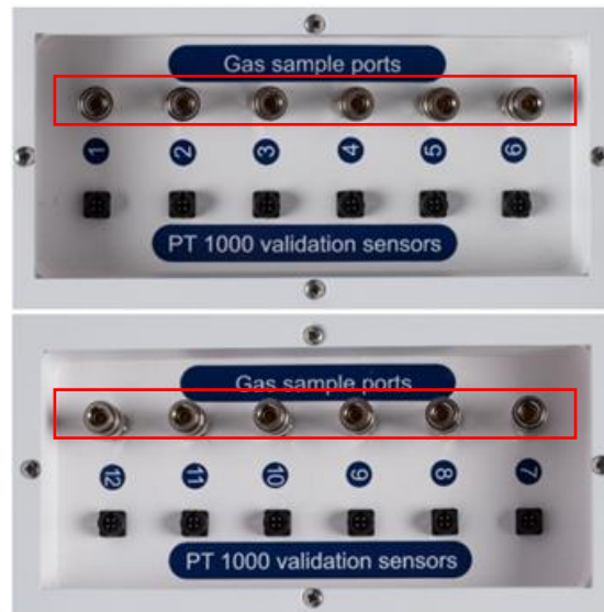
Figure 26.2 Gas sample ports in the MIRI® TL12 multiroom IVF incubator
