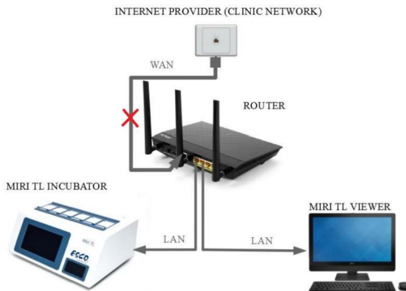
Figure 19.1 MIRI® TL family's multiroom incubator's connection scheme without the extended configuration package
