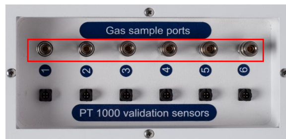
Figure 26.1 Gas sample ports in the MIRI® TL6 multiroom IVF incubator
